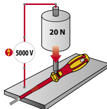
PRESSURE TEST (5000V)
